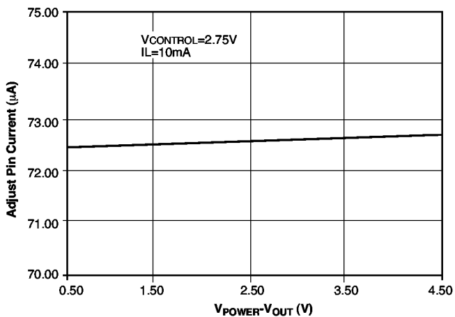
Adjust Pin Current vs V_{POWER}-V_{OUT}
