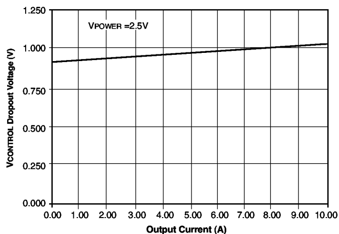
V_{CONTROL} Dropout Voltage vs I_{OUT}
