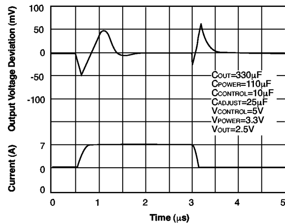
Current Step Transient Response
