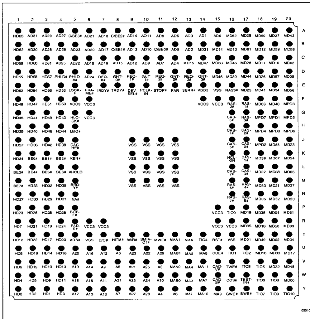
Figure 8. TxC Pinout
