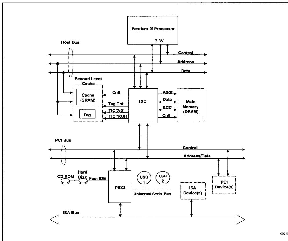
Figure 1. TxC System Block Diagram
