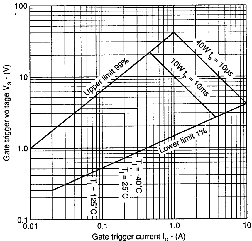
FIG. 2 GATE CHARACTERISTICS
