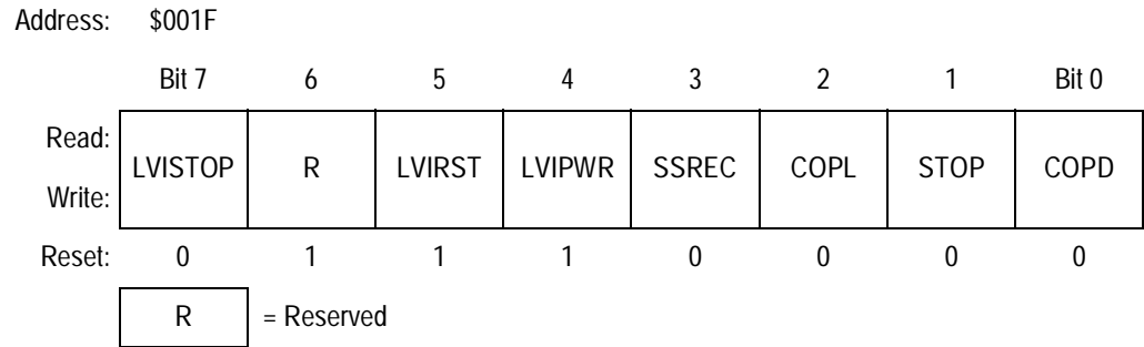
Figure 11-1. Configuration Write-Once Register (CONFIG-1)
