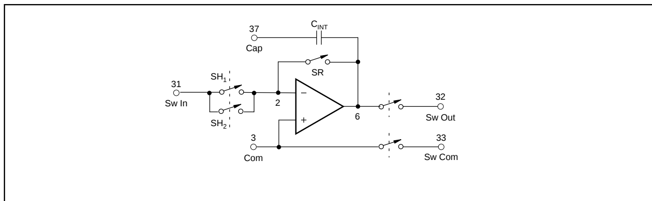
FIGURE C7. Node Assignments for ACF2101 Macromodel.
