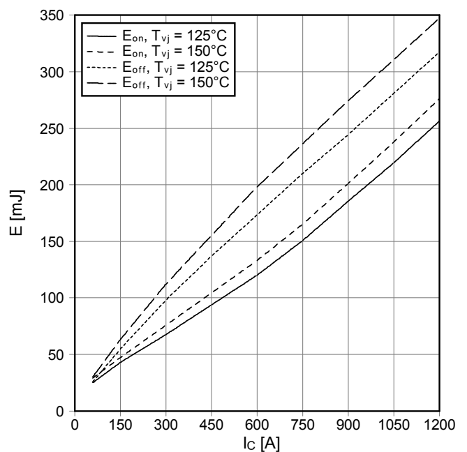
Schaltverluste IGBT-Wechselr. (typisch) switching losses IGBT-inverter (typical) E_{on} = f(I_c), E_{off} = f(I_c) V_{GE} = \pm 15\text{ V}, R_{Gon} = 1.2\ \Omega, R_{Goff} = 1.2\ \Omega, V_{CE} = 900\text{ V}
