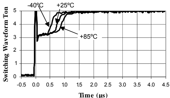
TX Off, 20 mA Load Current
