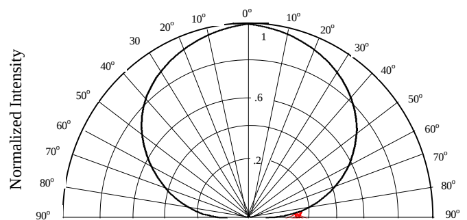
FIG 5. RADIATION DIAGRAM
