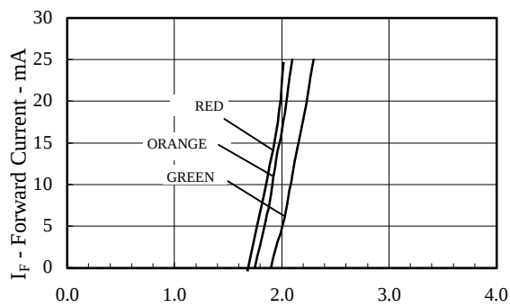
V_F - Forward Voltage - V FIG.2 FORWARD CURRENT VS. FORWARD VOLTAGE.
