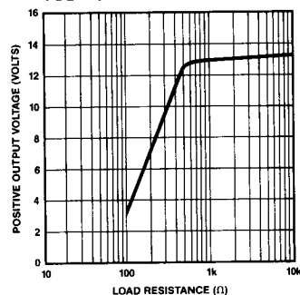
MAXIMUM POSITIVE OUTPUT VOLTAGE vs LOAD RESISTANCE
