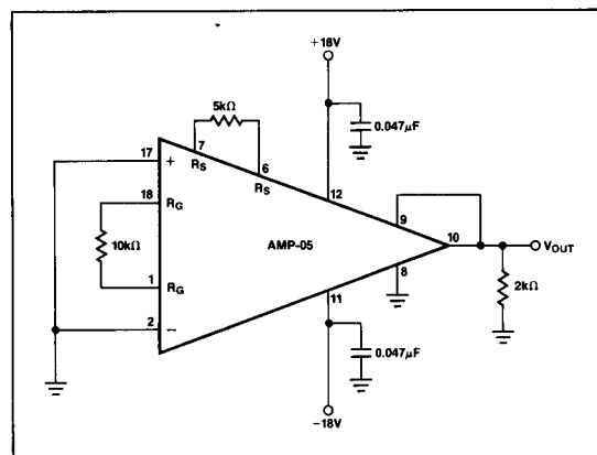
FIGURE 14: Burn-In Circuit
