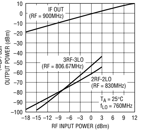
Low Band IF OUT, 2x2 and 3x3 Spurs vs RF Input Power (Single Tone)
