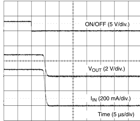
SiP4282-1 Turn-Off ( V_{IN} = 3 V, R_{LOAD} = 6 \Omega )
