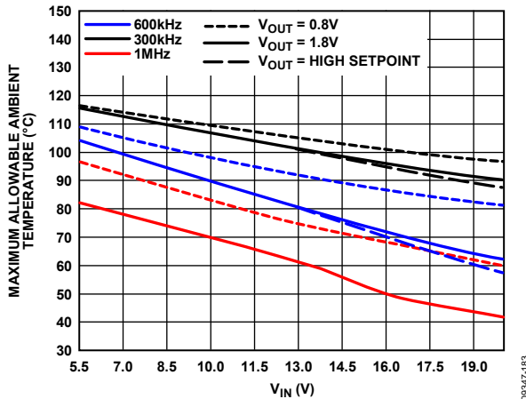
Figure 89. Ambient Temperature vs. V IN 4-Layer EVB, C IN = 4.3 nF (Upper-/Lower-Side MOSFET)
