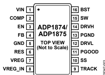
Figure 3. Pin Configuration
