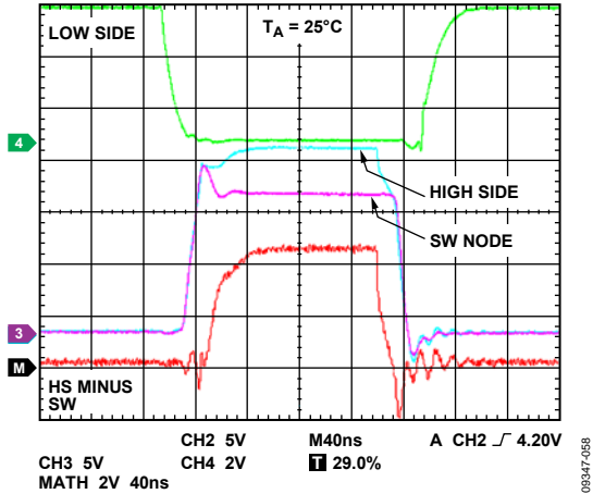
Figure 58. Output Drivers and SW Node Waveforms
