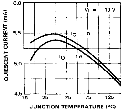
QUIESCENT CURRENT
