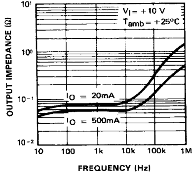
OUTPUT IMPEDANCE
