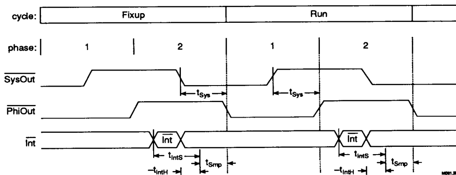
Figure 12.4 Interrupt Timing
