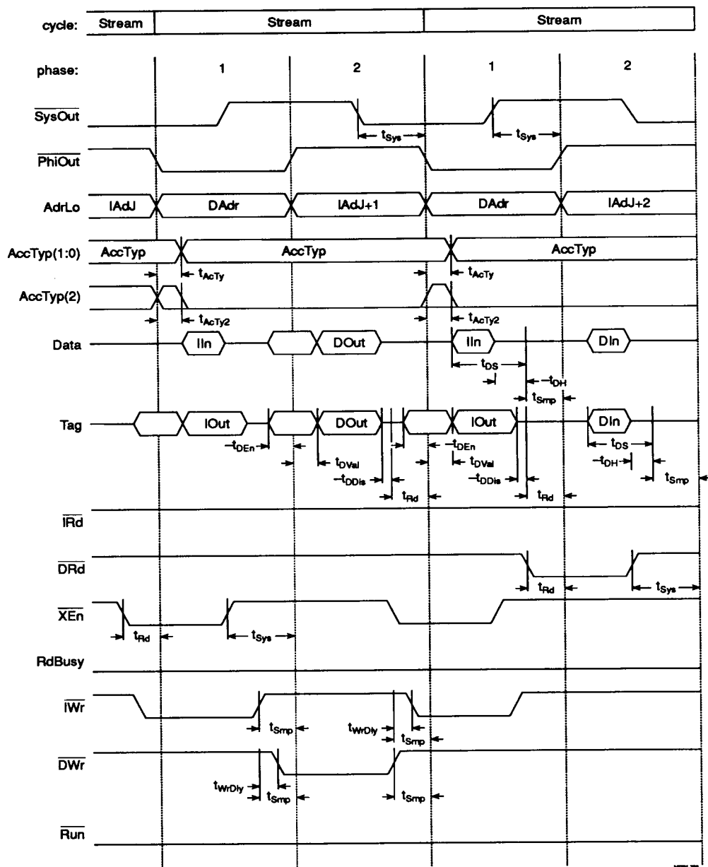
Figure 12.20 Instruction Stream, Stream-Stream
