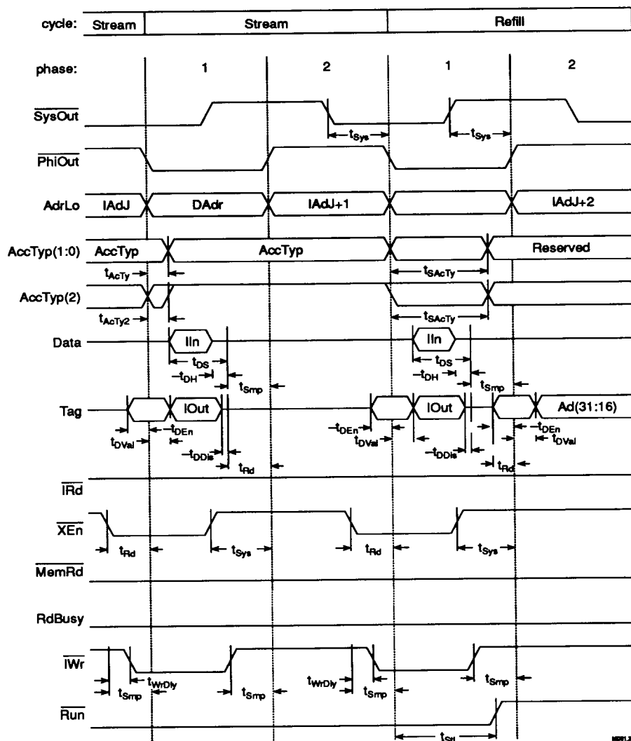
Figure 12.22 Instruction Stream, Stream-Refill
