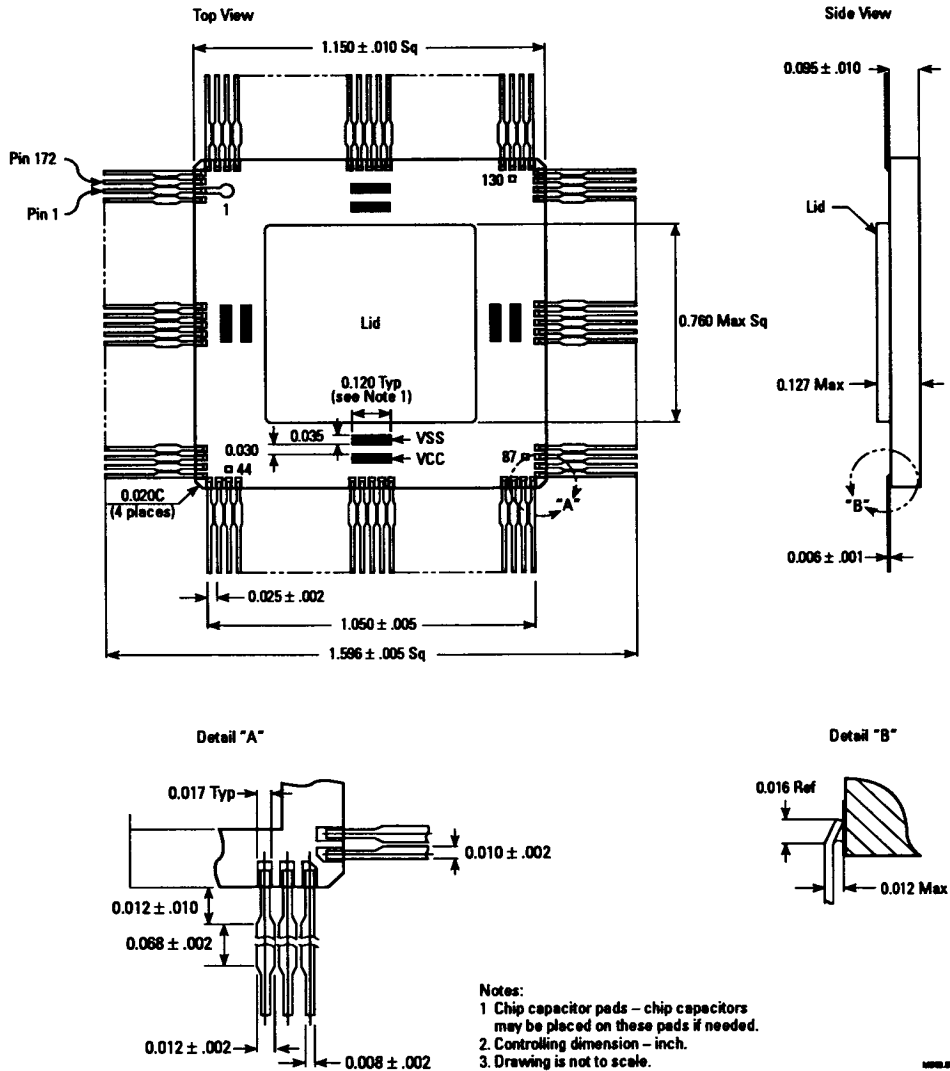
Figure 12.45 LR3000 Mechanical Drawing: 172-Pin Cavity-Up CLDCC
