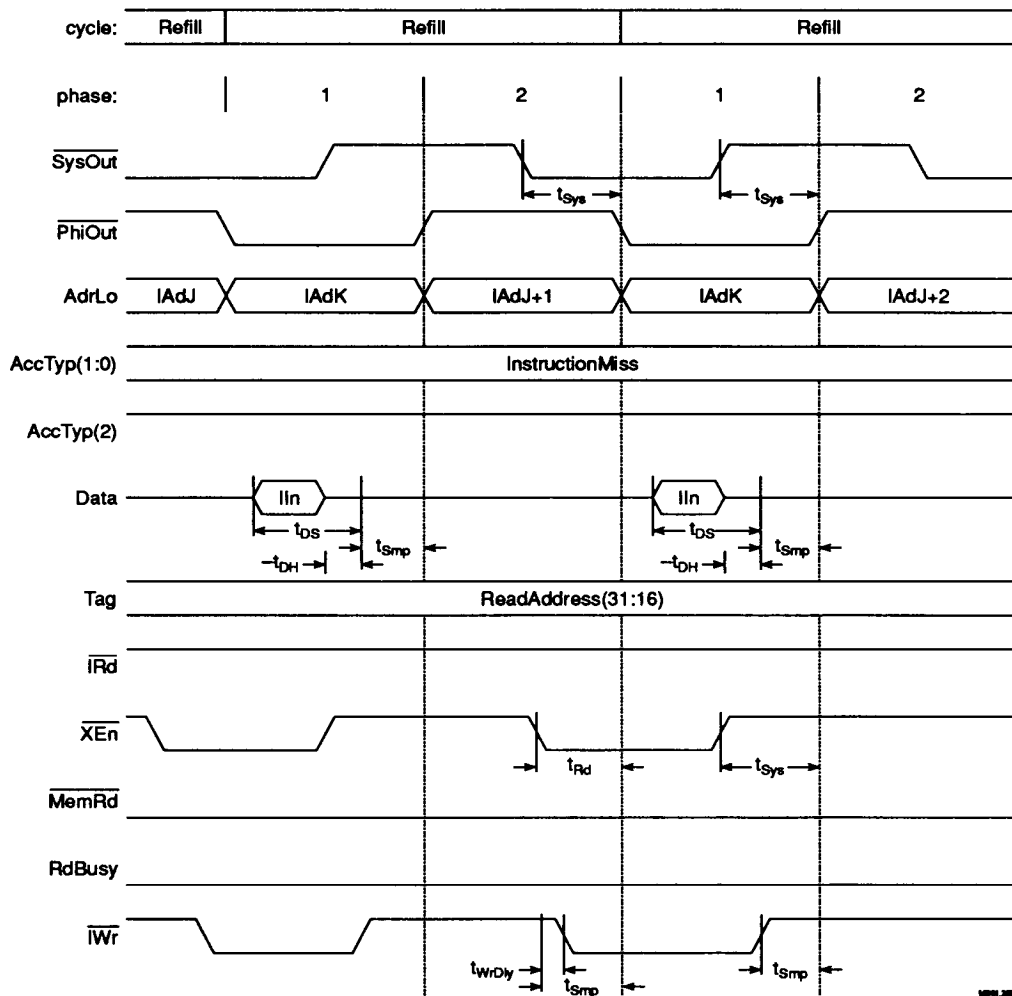
Figure 12.15 Instruction Block Transfer, Refill-Refill
