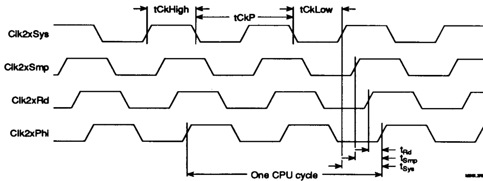
Figure 12.1 Clock Timing
