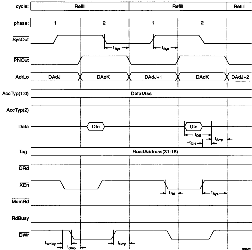
Figure 12.11 Data Block Transfer, Refill-Refill
