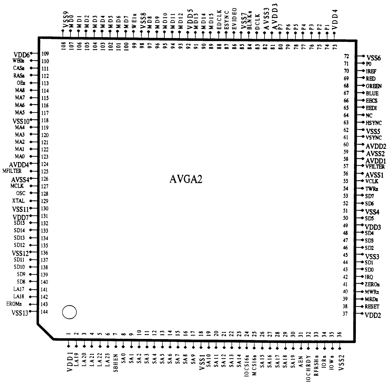
144 PIN PQFP pinout
