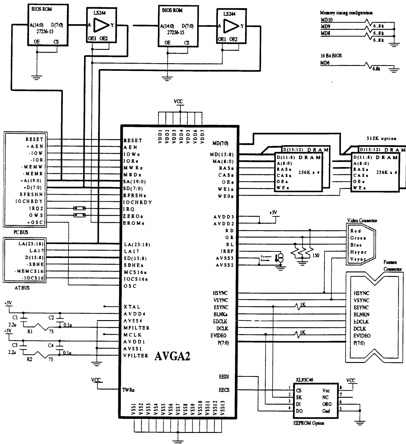
Typical PC/AT add-in 16 bit BIOS
