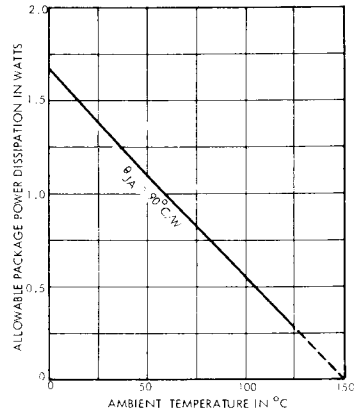
Dwg. No. A-10.884B
