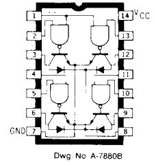
Dwg. No. A-7880B
