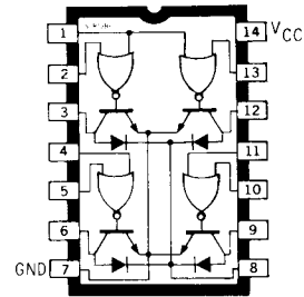
Dwg. No. A-9130B
