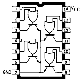
Dwg. No. A-12,389
