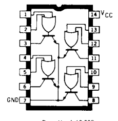
Dwg. No. A-12,389
