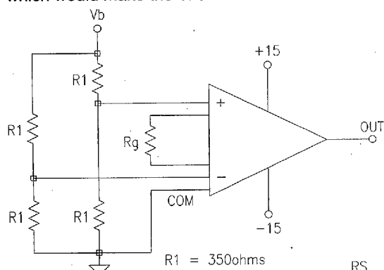
FIGURE 1. Basic Bridge Amplifier
