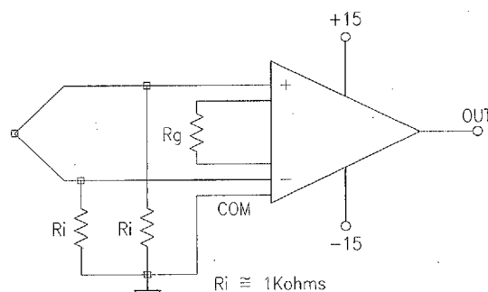
FIGURE 3. Thermocouple Amplifier
