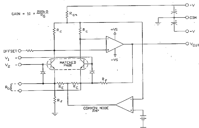
FIGURE 6. Simplified Schematic of Model 176
