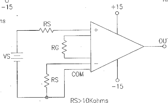
FIGURE 2. High Source Impedance Amplifier
