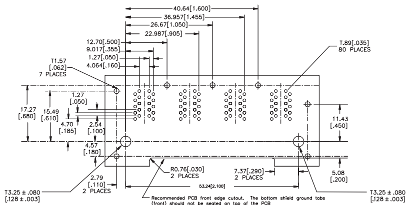
PC BOARD LAYOUT VIEWED FROM COMPONENT SIDE
