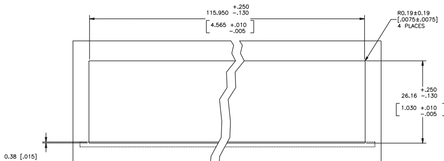
SUGGESTED PANEL CUTOUT DIMENSIONS
