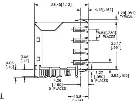
VIEW A - A
