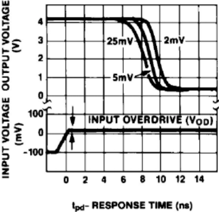
FIGURE 6. INPUT OVERDRIVE VS. t_{pd-} RESPONSE TIME
