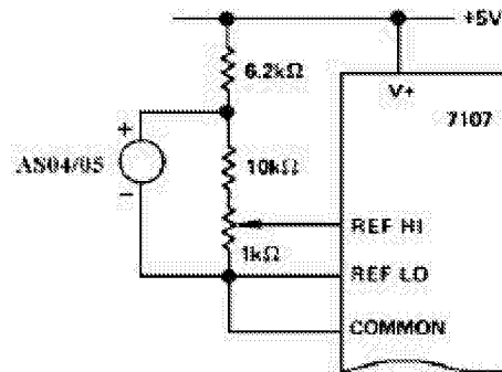
With 7107 Panel Meter A/D
