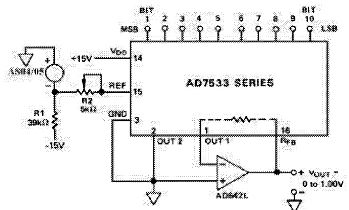
AS04/05 as Reference for 10-Bit CMOS DAC
