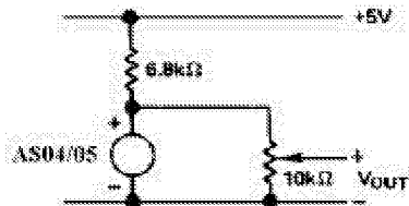
Basic Configuration for 1.2V or Less
