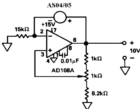
Single-Supply Buffered 10V Reference
