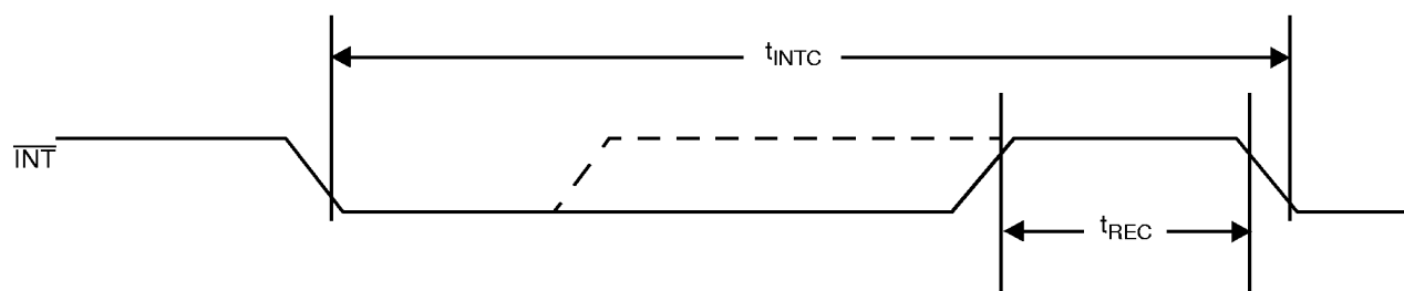
Figure 30. \overline{INT} Timing
