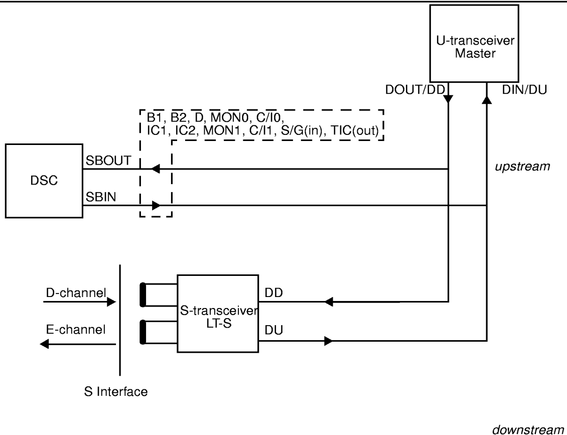
Figure 11. IOM-2 Intelligent Configuration
