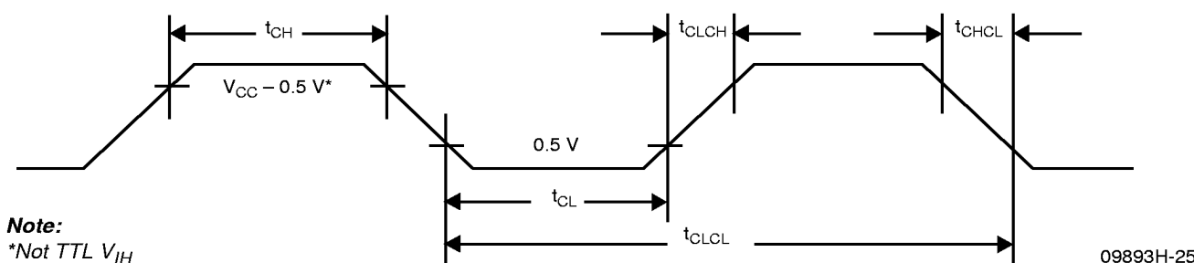
Figure 33. External Clock Driver (XTAL2) Timing
