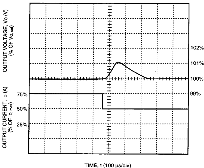
Figure 15. CC025 Triple-Output-Series Typical Output Voltage for a Step Load Change from 75% to 50% of Full Load on Output 1
