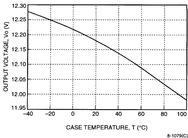
Figure 3. CC025 Triple-Output-Series Typical Output Voltage Variation of 12 V Output Over Ambient Temperature Range
