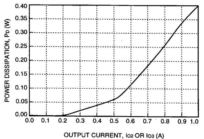
Figure 26. CC025ABK-M, Losses Associated with \pm 12 V Output, P_{s2}/P_{s3}
