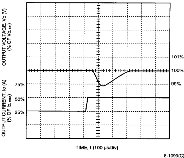
Figure 16. CC025 Triple-Output-Series Typical Output Voltage for a Step Load Change from 25% to 50% of Full Load on Output 1
