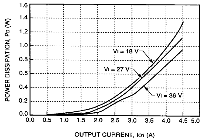
Figure 25. CC025ABK-M, CC025ACL-M Losses, Associated with 5 V Output, P_{s1}
