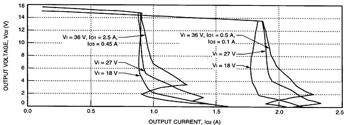
Figure 12. CC025ACL-M Typical 15 V Output Characteristics
