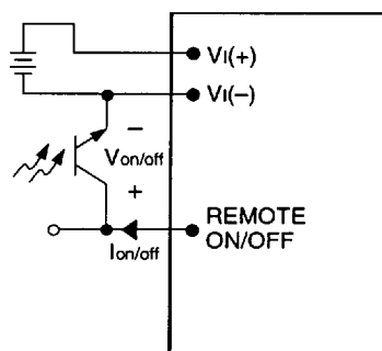
Figure 21. Remote On/Off Implementation
