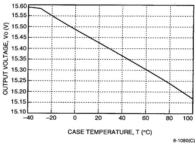
Figure 4. CC025 Triple-Output-Series Typical Output Voltage Variation of 15 V Output Over Ambient Temperature Range
