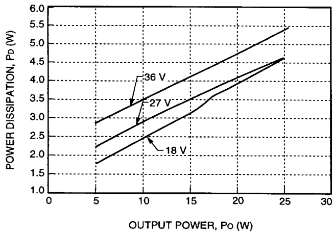
Figure 23. CC025ABK-M Fixed Losses, P_p
