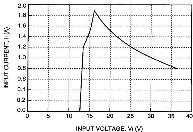
Figure 1. CC025 Triple-Output-Series Typical Input Characteristics
