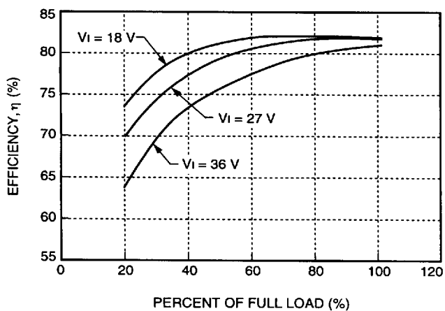
Figure 12. CC025ACL-M Typical 15 V Output Characteristics
