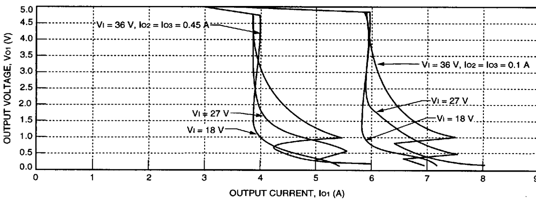
Figure 11. CC025ACL-M Typical 5 V Output Characteristics
