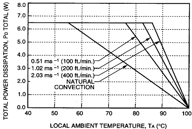
Figure 28. Total Power Dissipation vs. Local Ambient Temperature and Air Velocity
