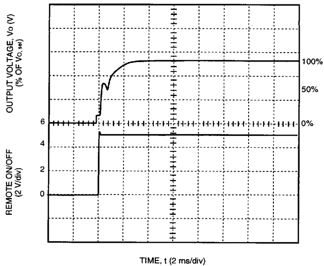
Figure 17. CC025 Triple-Output-Series Typical Output Voltage Start-Up when Signal Applied to Remote On/Off
