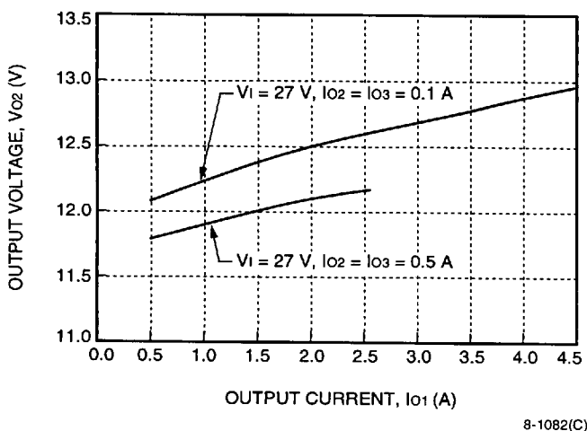
Figure 6. CC025ABK-M Typical Cross Regulation with Respect to I_{01}
