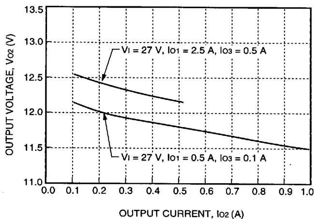
Figure 5. CC025ABK-M Typical Load Regulation
