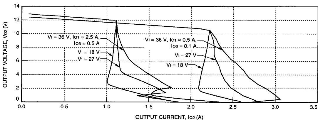
Figure 10. CC025ABK-M Typical 12 V Output Characteristics
