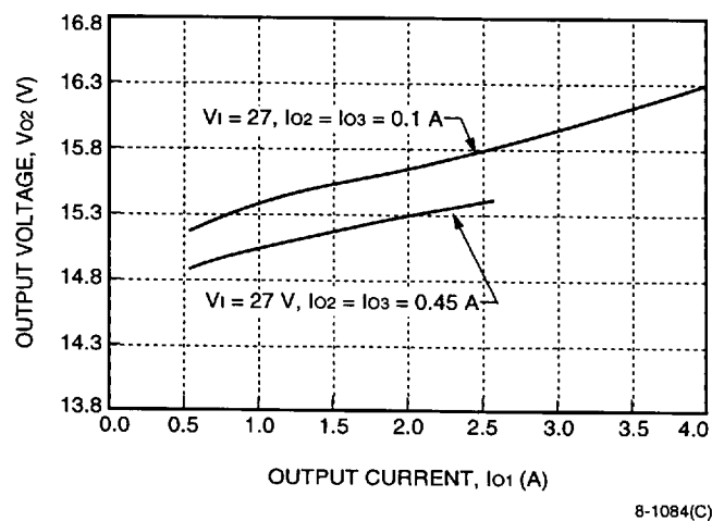
Figure 8. CC025ACL-M Typical Cross Regulation with Respect to I_{01}
