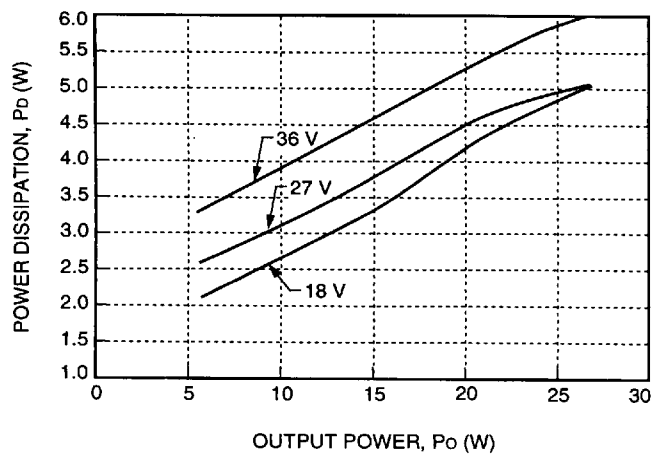
Figure 24. CC025ACL-M Fixed Losses, P_p
