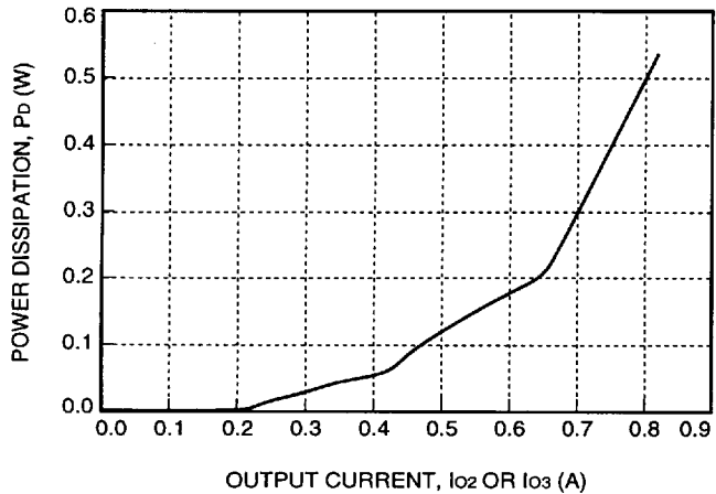
Figure 27. CC025ACL-M Losses Associated with \pm 15 V Output, Ps2/Ps3
