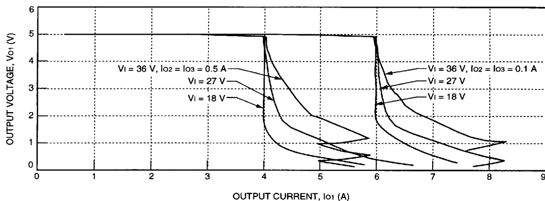
Figure 9. CC025ABK-M Typical 5 V Output Characteristics
