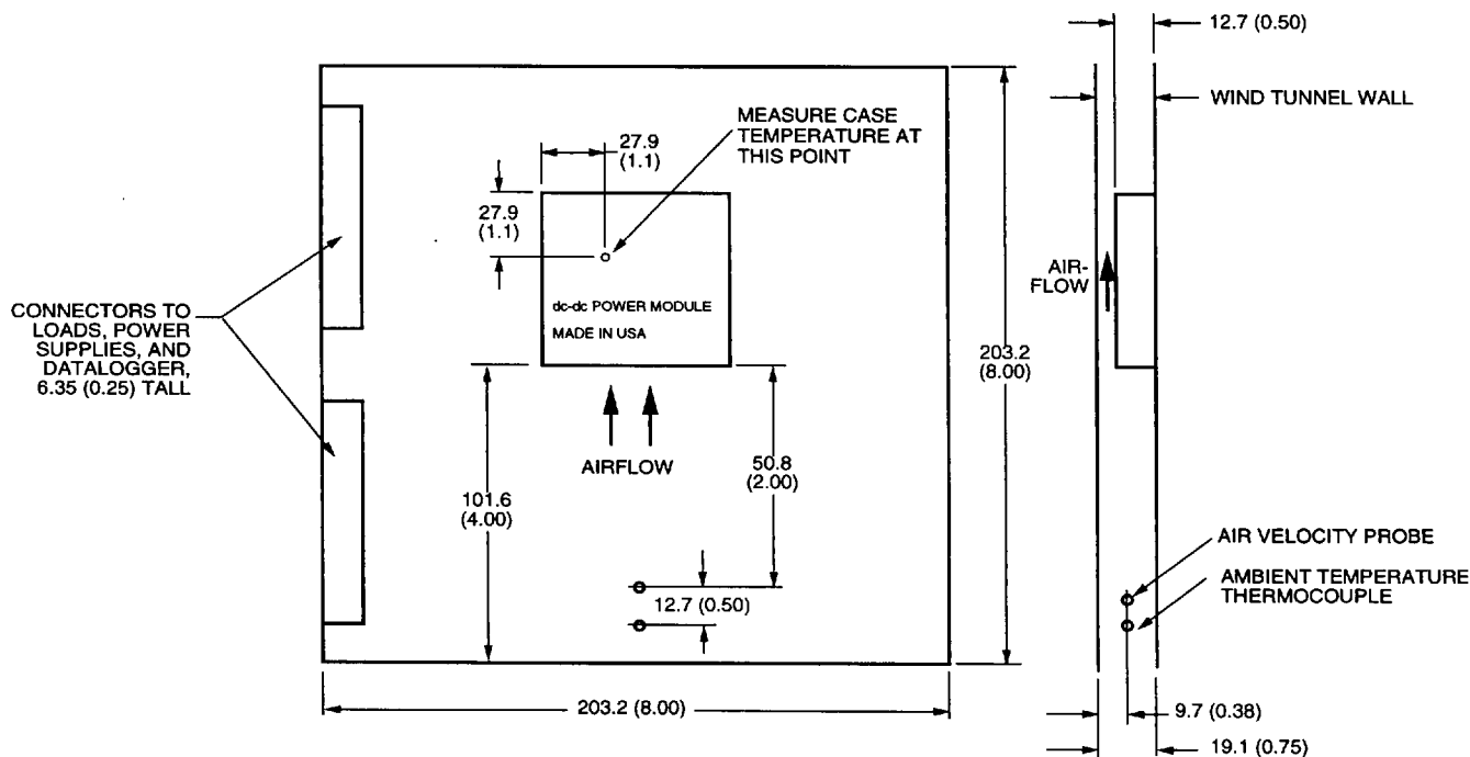
Figure 22. Thermal Test Setup
