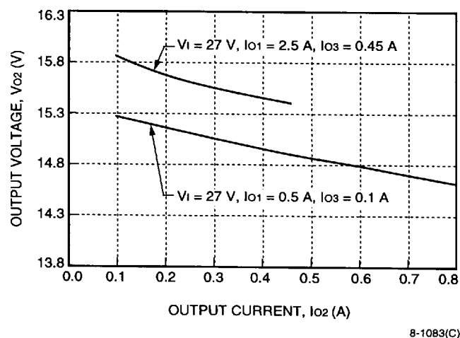
Figure 7. CC025ACL-M Typical Load Regulation
