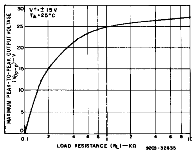
Fig. 7 - Output voltage as a function of load resistance.
