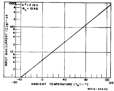
Fig. 14 - Input bias current as a function of ambient temperature.
