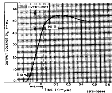
Fig. 16 - Output voltage as a function of elapsed time.
