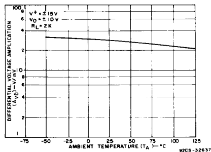
Fig. 9 - Differential voltage amplification as a function of ambient temperature.
