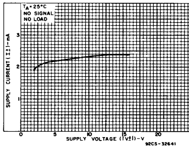
Fig. 13 - Supply current as a function of supply voltage.
