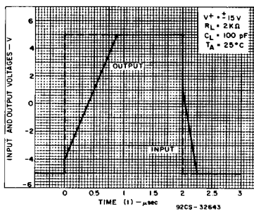
Fig. 15 - Voltage follower large-signal pulse response.
