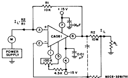
Fig. 21 - Basic current amplifier for low-current measurement systems.
