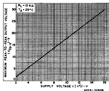
Fig. 8 - Output voltage as a function of supply voltage.
