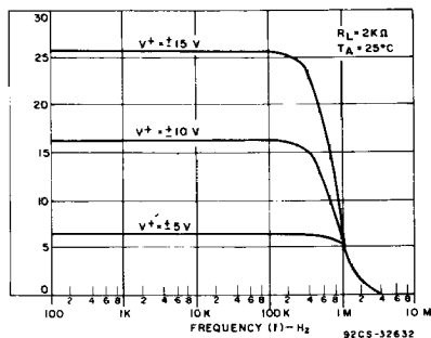
Fig. 5 - Output voltage as a function of frequency.
