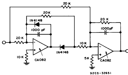
Fig. 20 - Unity-gain absolute-value amplifier.
