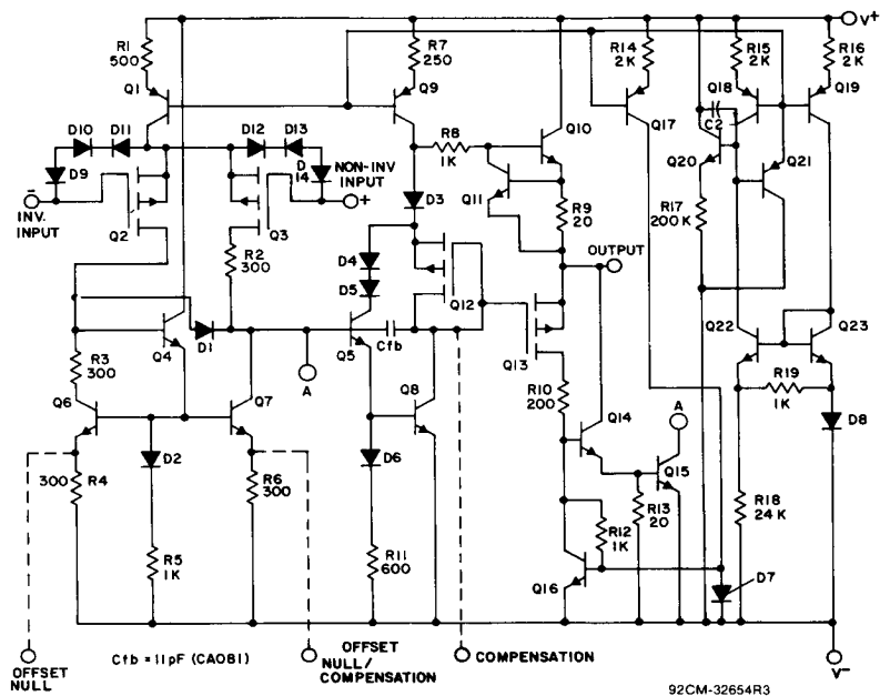
Fig. 1 - Schematic diagram of the CA081, CA082, and CA084.
