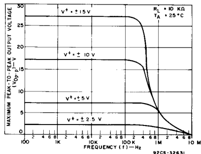
Fig. 4 - Output voltage as a function of frequency.
