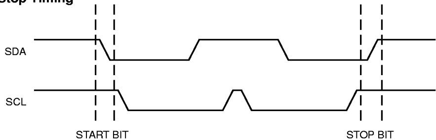
Figure 3. Start/Stop Timing
