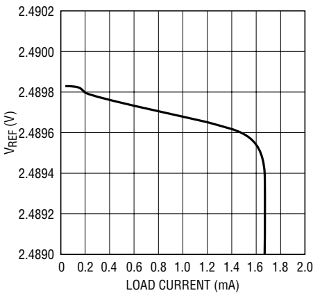
Internal Reference Voltage vs Load Current
