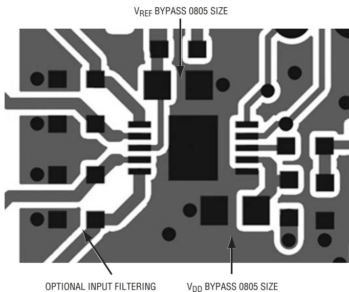
Figure 5. Recommended Layout
