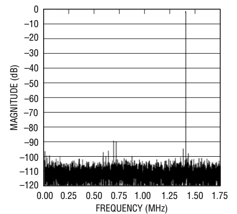
1.4MHz Sine Wave 8192 Point FFT Plot
