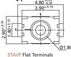
STAVF_15 Height=1.5mm
