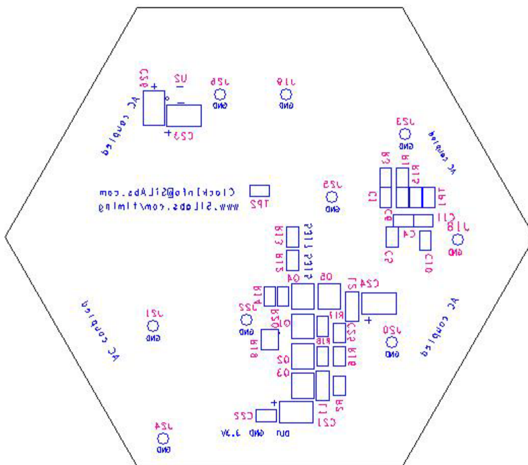
Figure 12. Bottom Silkscreen
