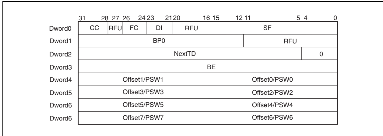
Figure 14-12. IsochronousTD Format
