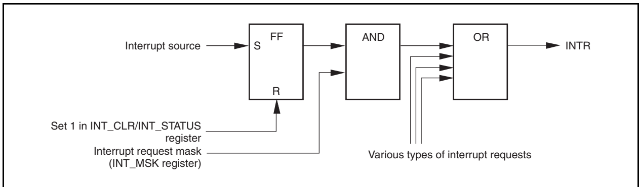
Figure 15-9. Interrupt Control
