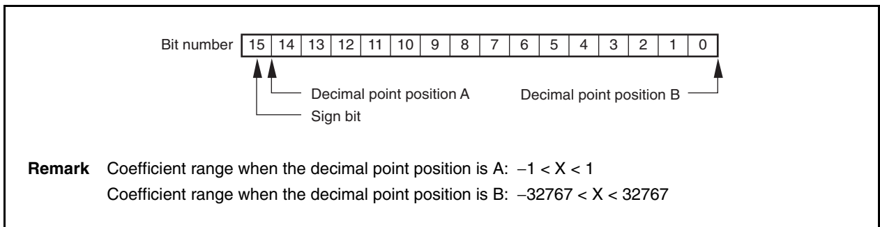
Figure 15-10. Input Data
