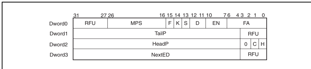
Figure 14-9. ED Format
