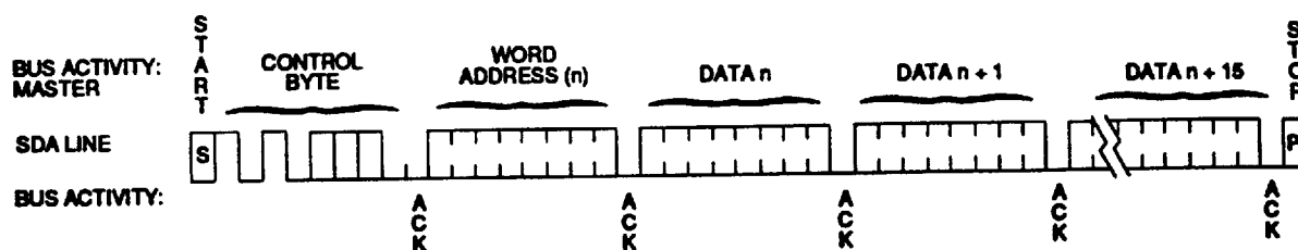
FIGURE 4 - PAGE WRITE
