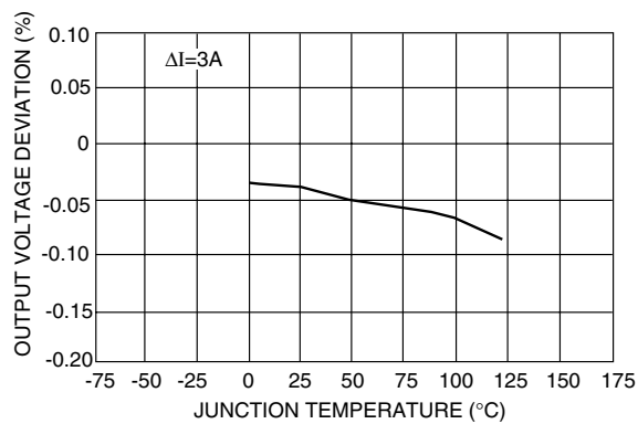
Load Regulation vs. Temperature
