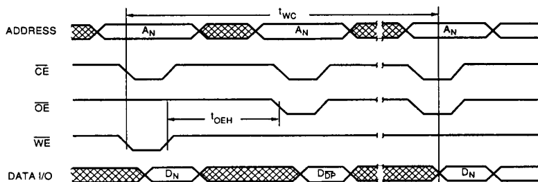
FIGURE 6. DATA POLLING TIMING
