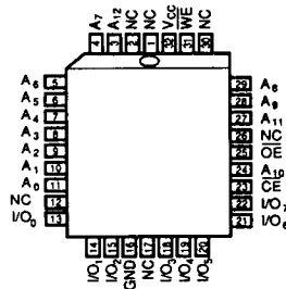
32 Pin PLCC Type "D" Package
