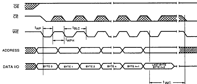
FIGURE 5. PAGE MODE WRITE CYCLE TIMING
