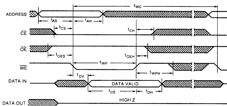
FIGURE 3. WE CONTROLLED WRITE CYCLE TIMING
