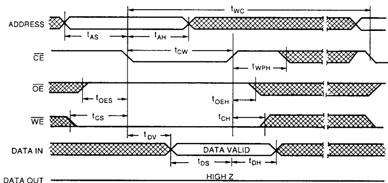
FIGURE 4. CE CONTROLLED WRITE CYCLE TIMING
