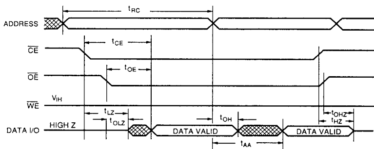
FIGURE 2. READ CYCLE TIMING
