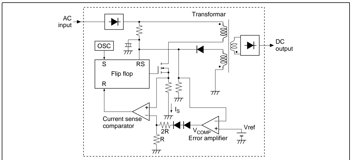
Figure 5 Block Diagram of Current Mode Switching Power Supply
