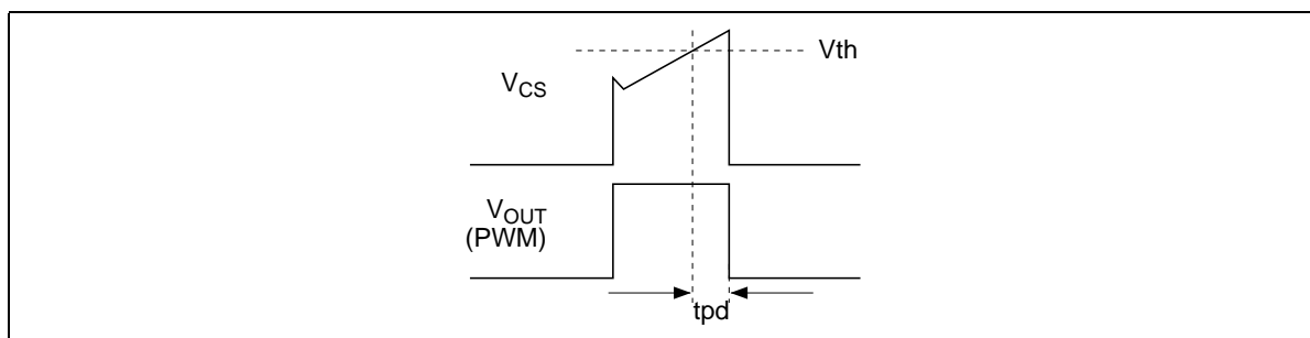
Figure 1 Definition of Current Sensing Response Time tpd
