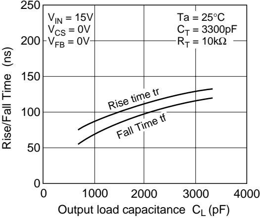
Rise/Fall Time of Output Pulse vs. Load Capacitance
