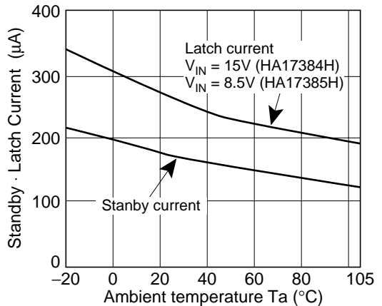
Standby Current/Latch Current vs. Ambient Temperature
