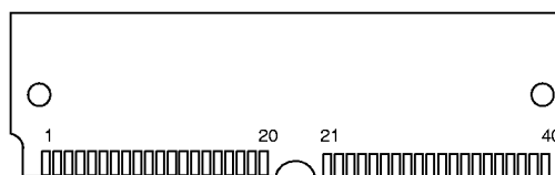
40-PIN SIMM
