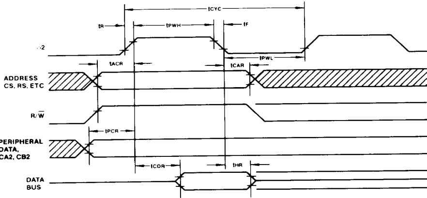
Figure 2. Read Timing
