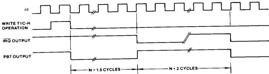
Figure 26. Free-Run Mode (Timer 1)
