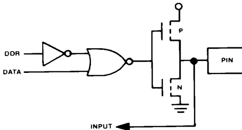
Figure 14. Port A Buffer Circuit (PA0-PA7, CA2)
