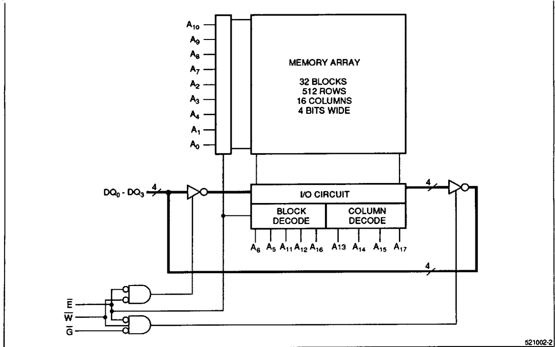
Figure 2. LH521002 Block Diagram
