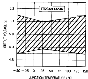
Worst Case Output Voltage
