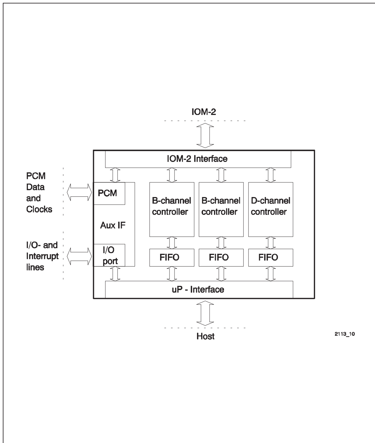
Figure 3 Block Diagram
