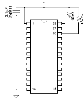
Figure 4: AutoStore ™ Inhibit Mode
