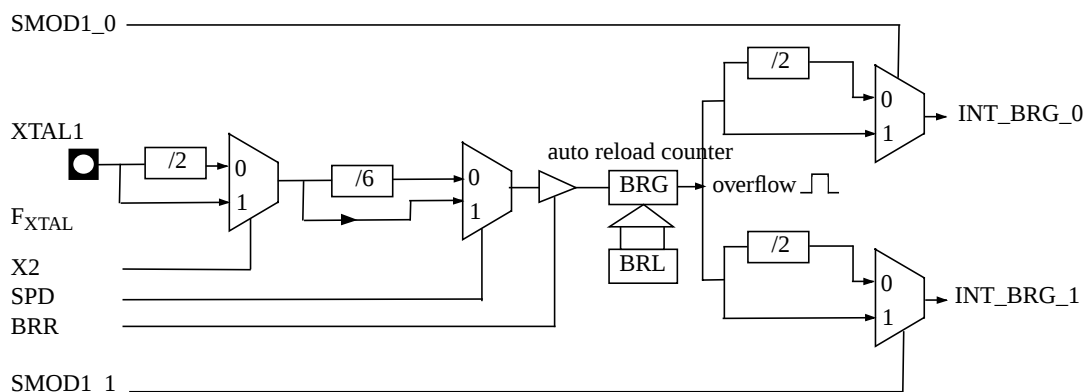
Figure 11. Internal Baud Rate
