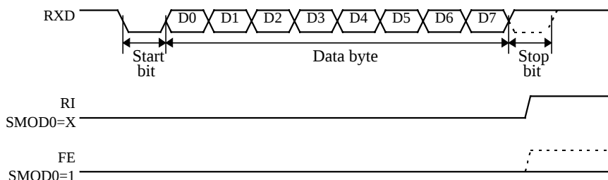
Figure 7. UART Timings in Mode 1
