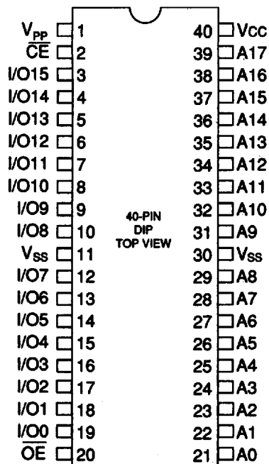
HN27C4096HG Series
