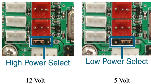
Figure 10: High / Low Power Select
