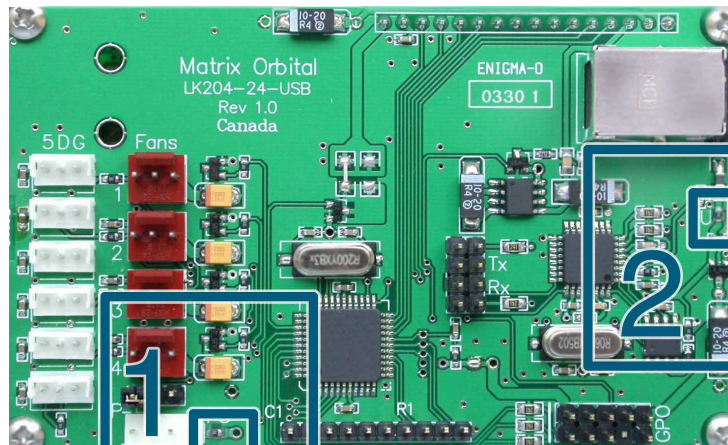
Figure 4: Jumper Locations
