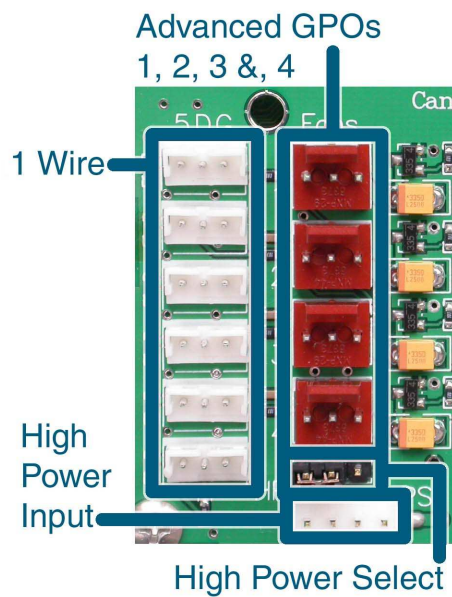
Figure 9: GPOs 1 to 4
