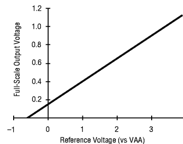
Figure 5. Full-Scale Output Voltage vs. V_{REF}
