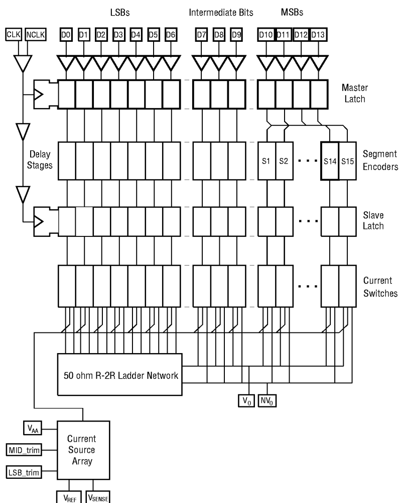
Figure 1. TQ6124 Block Diagram
