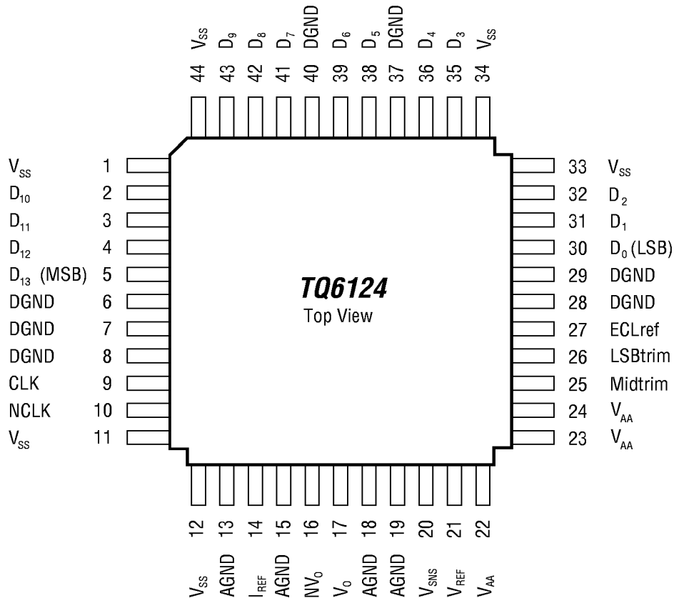
Figure 6. TQ6124 Pinout
