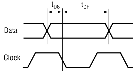
Figure 3. AC Timing Relationships
