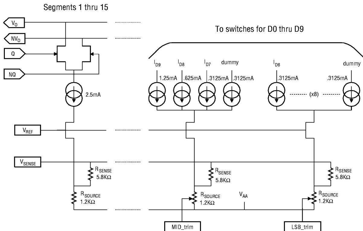
Figure 2. TQ6124 Currents
