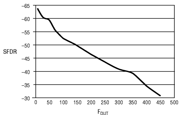
Figure 7. SFDR vs. Output Frequency
