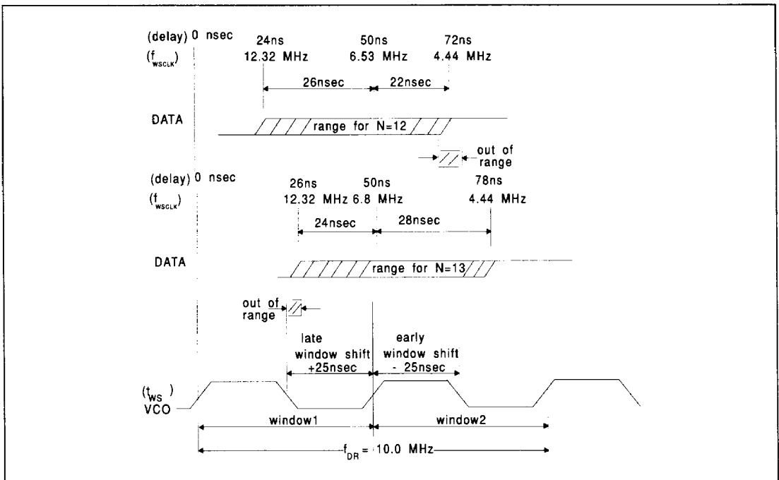
FIGURE 6. AWS NON-OPTIMUM FREQUENCY
