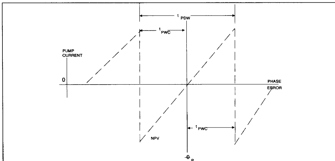
FIGURE 9. PHASE DETECTION TIMING
