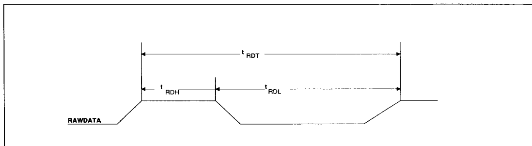
FIGURE 7. DISK DRIVE RAW READ DATA TIMING
