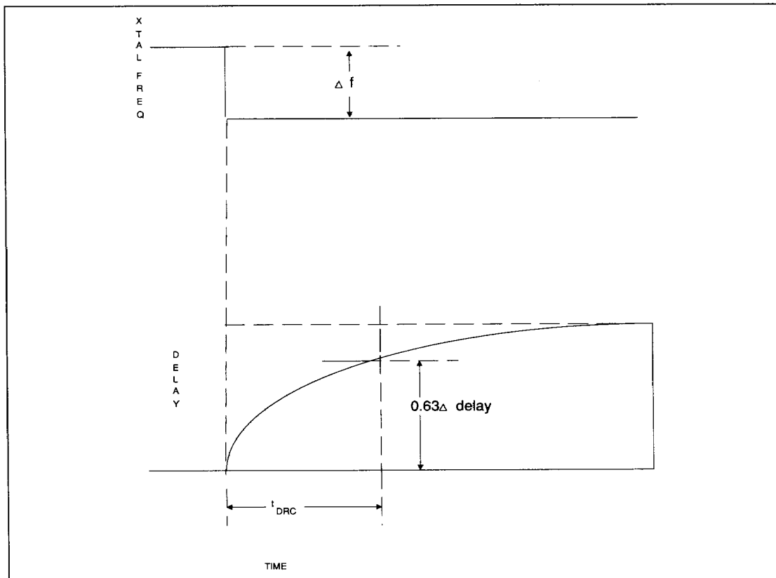
FIGURE 12. DELAY LINE TIMING
