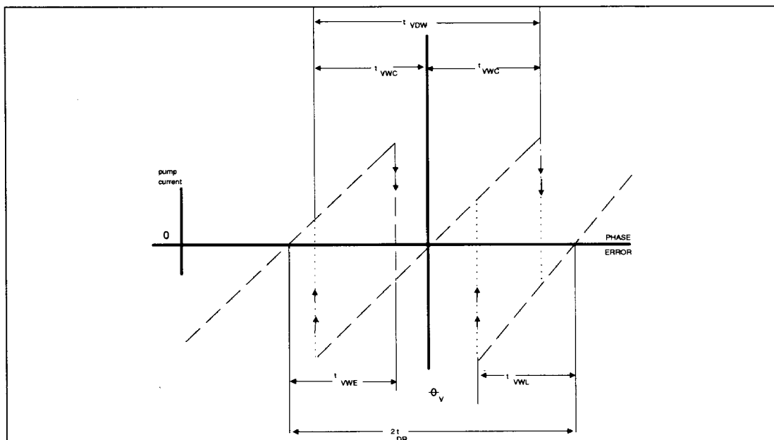
FIGURE 10. VELOCITY LOCK MODE
