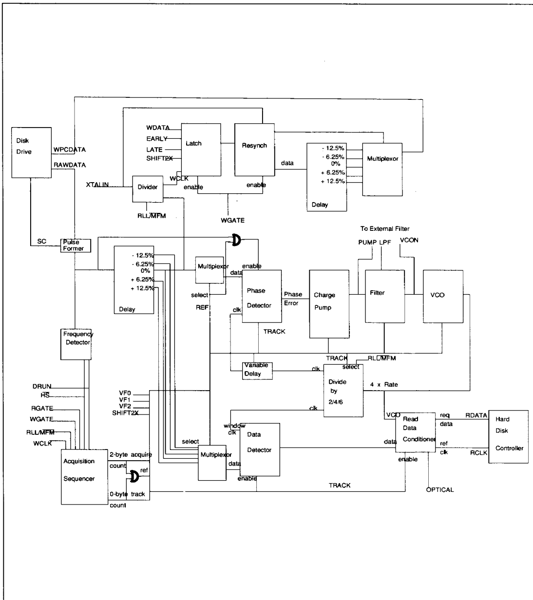
FIGURE 3. WD10C23 BLOCK DIAGRAM
