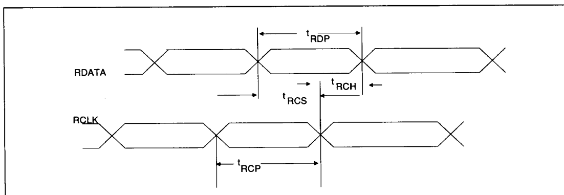
FIGURE 8. READ DATA CONDITIONER TIMING
