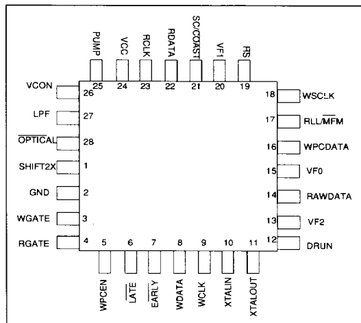
FIGURE 2. PIN DESIGNATION (QUAD)
