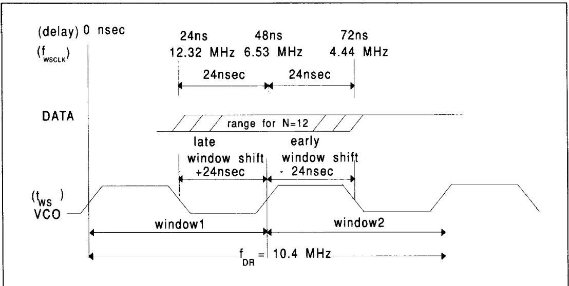
FIGURE 5. AWS OPTIMUM CENTER FREQUENCY
