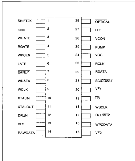
FIGURE 1. PIN DESIGNATION (DIP)
