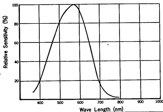
Fig3 Spectral Response
