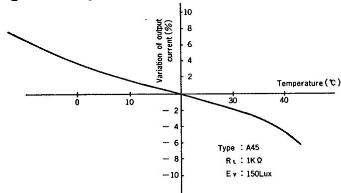
Fig4 Temperature Coefficient
