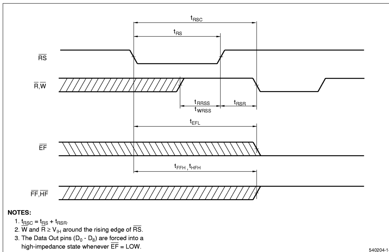
Figure 10. Reset Timing
