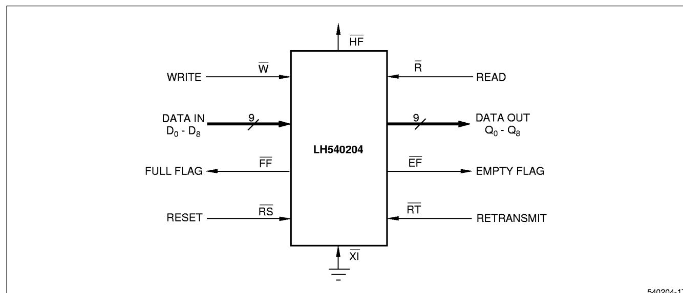
Figure 4. Standalone FIFO (4096 × 9)
