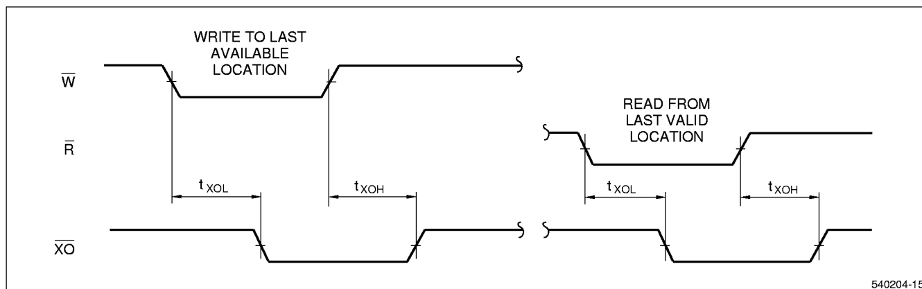
Figure 20. Expansion-Out Timing
