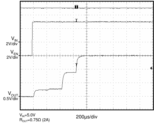
Start Up (Enable)( V_{OUT}=1.5V )
