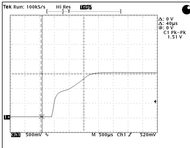
Figure 25. 1.5V Start-up characteristic at V_{IN} = 48\text{Vdc} , full load condition at T_A = 25^\circ\text{C} .
