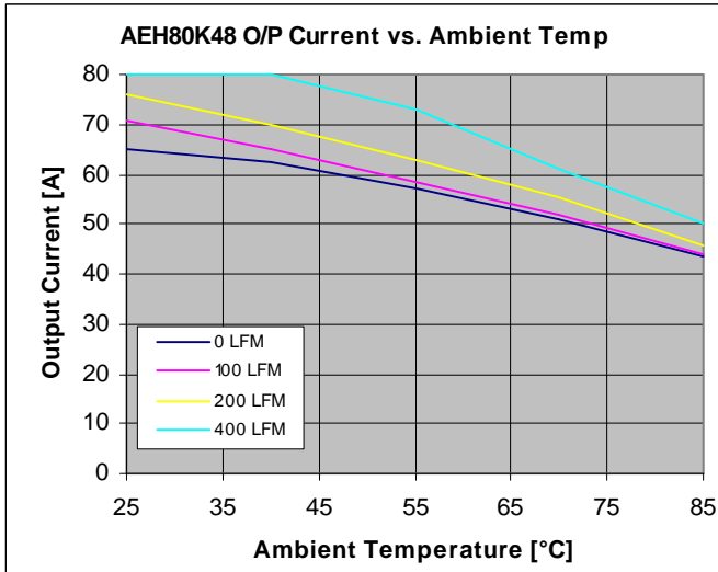
Figure 21. 1.2V Output Derating Curves (100°C Baseplate) at various airflow conditions directed across PIN 4 to 1 with the module mounted vertically.
