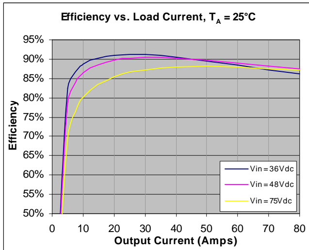
Figure 5. Efficiency vs. Load Current Curves at T A =25°C for different input voltages with 300 LFM airflow directed from Pins 4 to 1.
