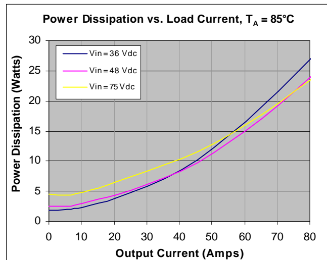
Figure 8. Power Dissipation vs. Load Current at T A =85°C for different input voltages with 300LFM airflow directed from Pins 4 to 1.
