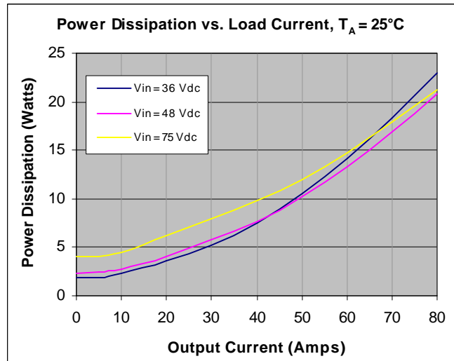
Figure 6. Power Dissipation vs. Load Current Curves at T A =25°C for different input voltages with 300 LFM airflow directed from Pins 4 to 1.
