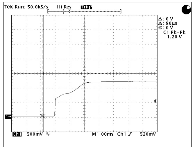
Figure 27. 1.2V Start-up characteristic at V_{IN} = 48\text{Vdc} , full load condition at T_A = 25^\circ\text{C} .
