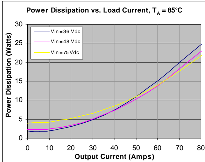
Figure 16. Power Dissipation vs. Load Current at T_A=85^\circ\text{C} for different input voltages with 300 LFM airflow directed from Pins 4 to 1.
