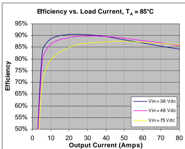
Figure 7. Efficiency vs. Load Current Curves at T A =85°C for different input voltages with 300 LFM airflow directed from Pins 4 to 1.
