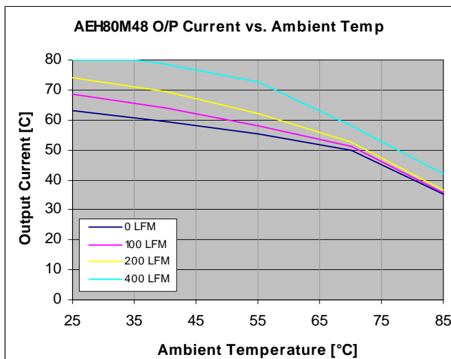
Figure 19. 1.5V Output Derating Curves (100°C Baseplate) at various airflow conditions directed across PIN 4 to 1 with the module mounted vertically.
