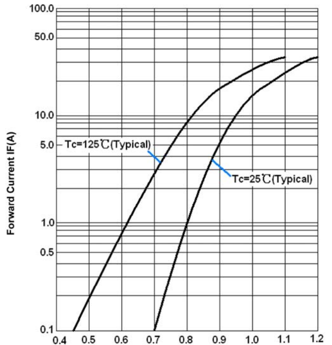
Fig.4 Forward Voltage
