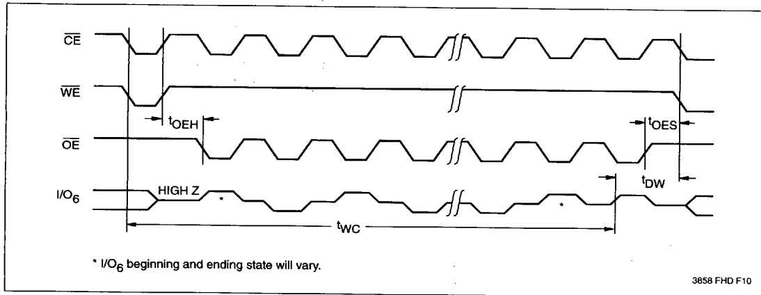
Toggle Bit Timing Diagram
