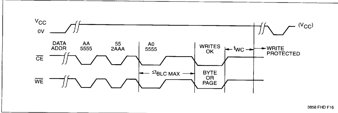
Figure 7. Write Sequence for Software Data Protection
