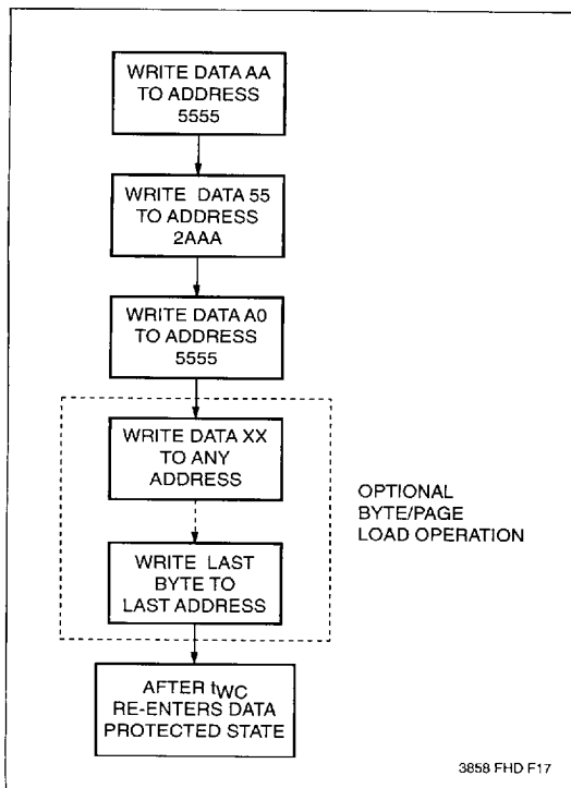
Figure 7. Write Sequence for Software Data Protection
