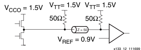
Figure 48: Terminated HSTL Class IV
